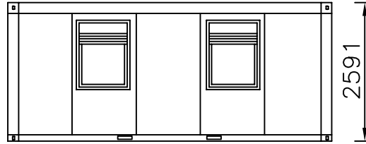
FRONT VIEW 1:100
